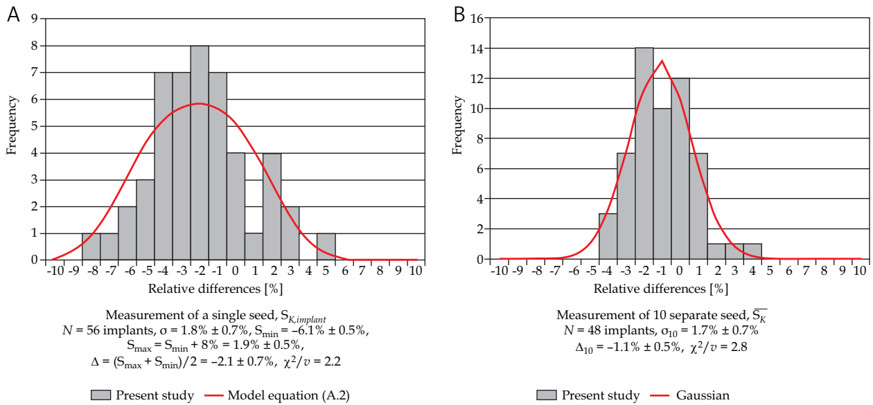
Fig. 4. A) (S_{K, implant} - S_K^C_i) / S_K^C_i for 56 implants has been fitted to the model of equation (A.2). The fitted parameters are \sigma and S_{min} . The model assumes one measurement for both the manufacturer and the user. B) (\bar{S}_K - S_K^C_i) / S_K^C_i distribution for 48 of 56 implants. The fitted parameters are \sigma_{10} and \Delta_{10}
