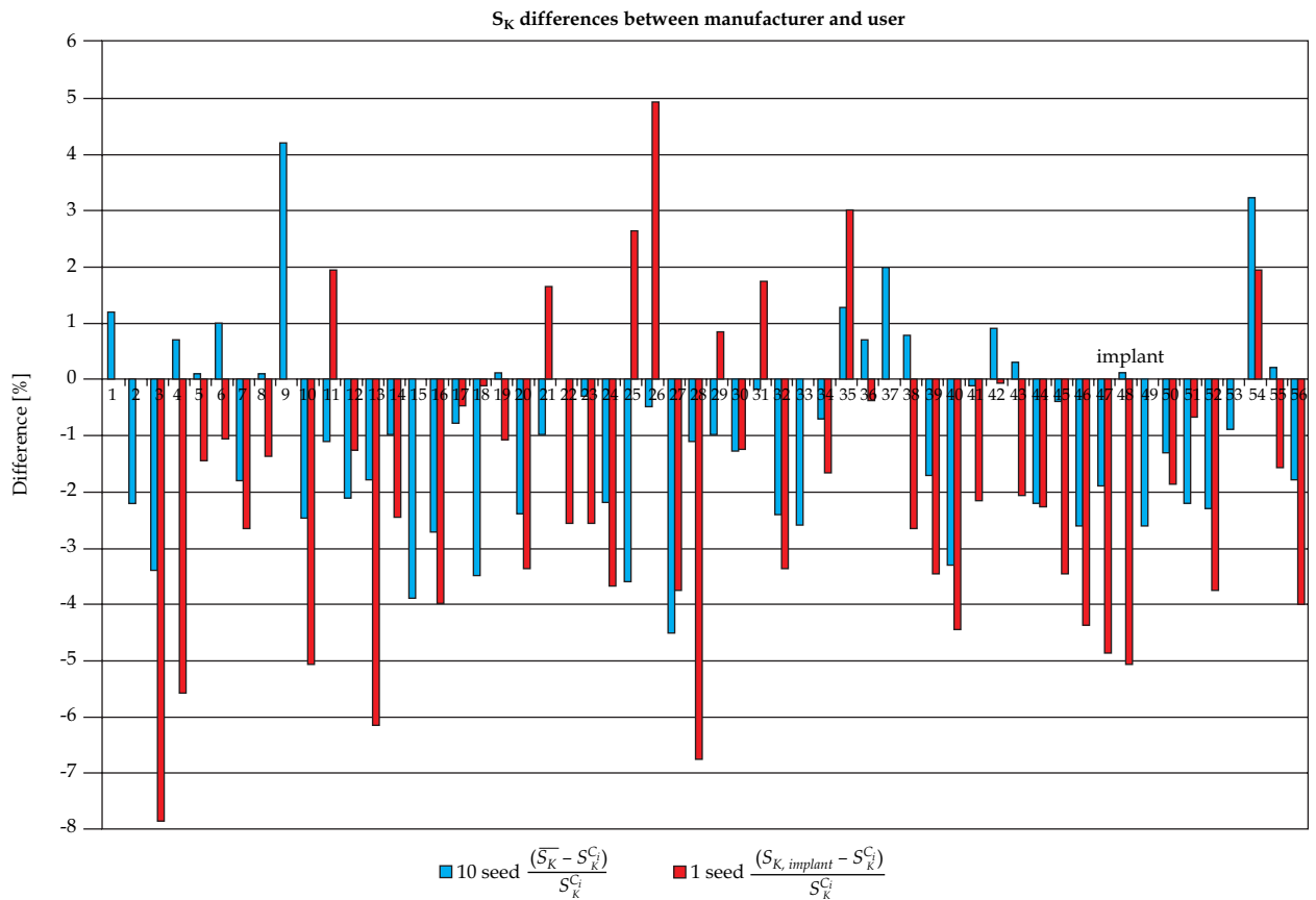
Fig. 3. (S_{K, implant} - S_K^C_i) / S_K^C_i and (\bar{S}_K - S_K^C_i) / S_K^C_i for 56 implants. In some implants the measurement of one seed was not done because all seeds were used in the implant
