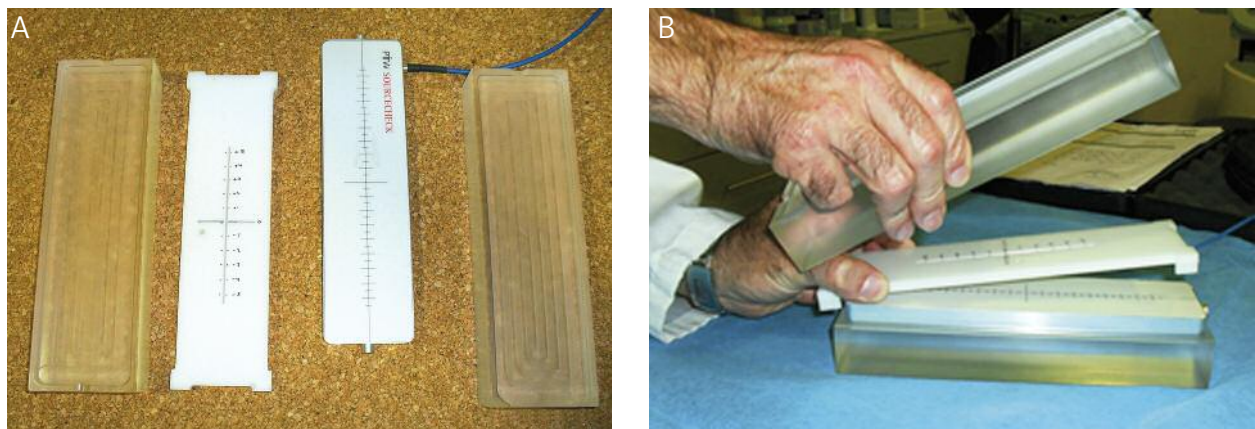
Fig. 1. A) Left-right: PMMA block, Nucletron insert to allocate the 10 selectSeed™, PTW SourceCheck (without the PTW insert), PMMA block (B) Mounting the set-up. Bottom-top: PMMA block + SourceCheck + Nucletron insert + PMMA block
